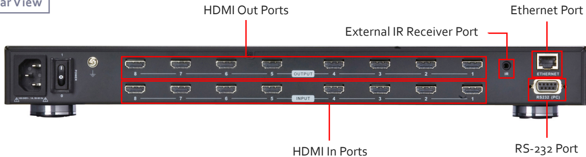
Rear View
