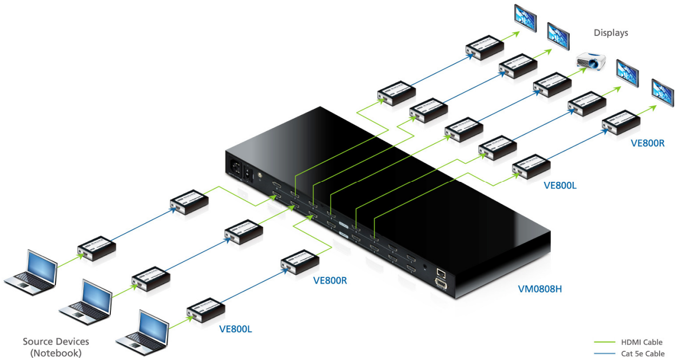
VM0808H x 1 8x8 HDMI Matrix Switch
