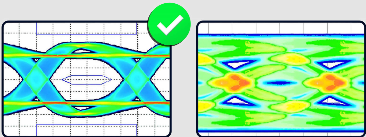
ATEN-Fair Eye Pattern
