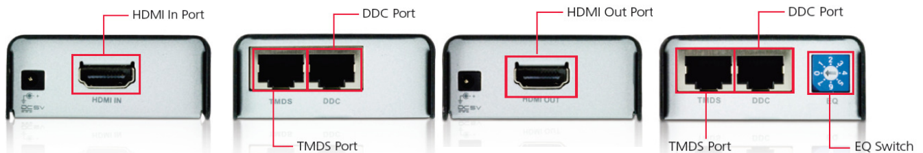
Front View
