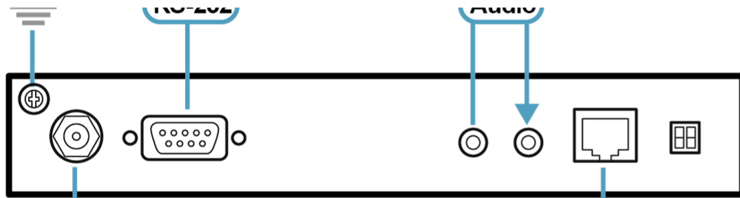
CE824L Rear View
