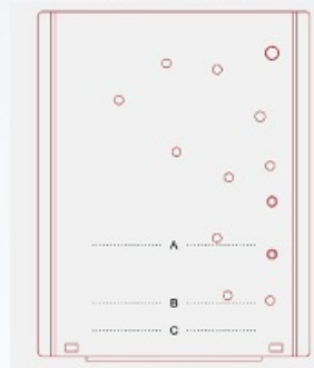
Mounting Plate
