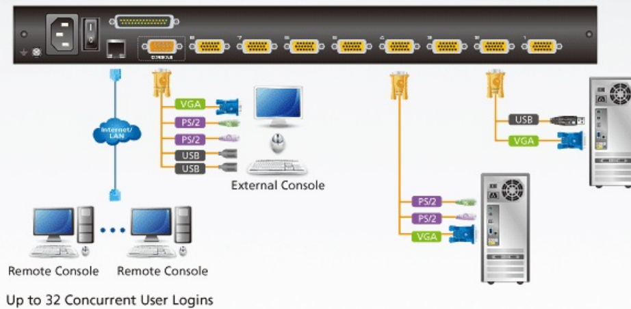
CL5708I (Rear)
