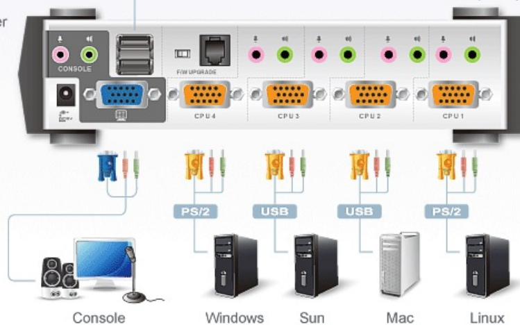
CS1734A (Rear)
