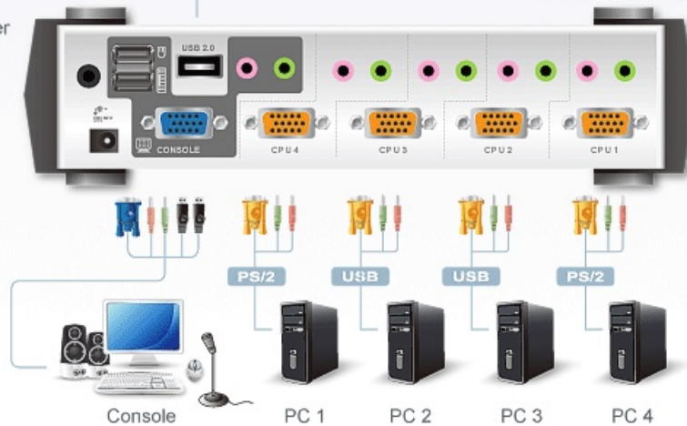
CS1734B (Rear)
